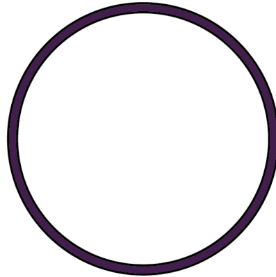
Charged shell
