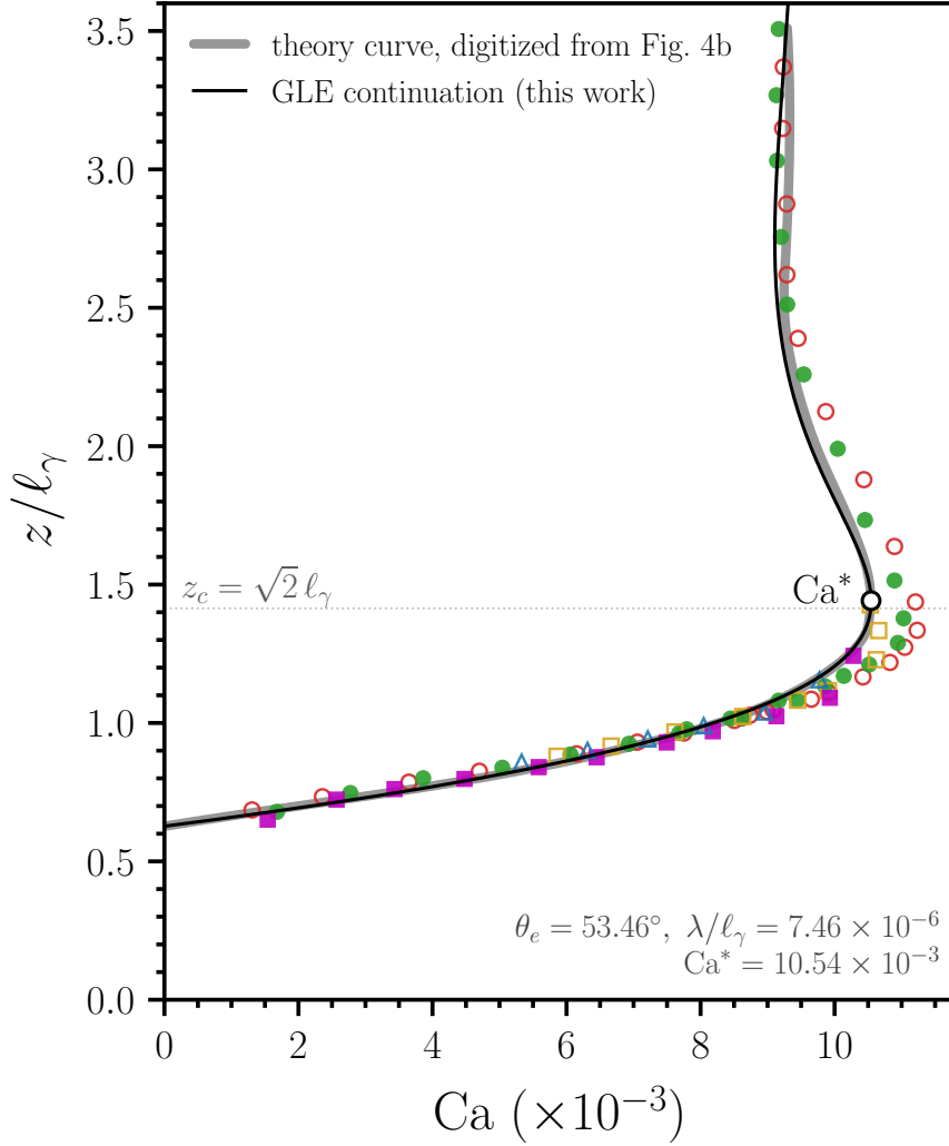
Figure 1: Steady meniscus rise at a receding contact line. Normalised contact-line elevation z/\ell_\gamma against capillary number Ca = \eta U_p/\gamma for a partially wetting plate withdrawn from a silicone-oil bath. The black line is the present GLE continuation; the thick grey line is the multiscale-lubrication prediction digitised from Fig. 4b of Snoeijer & Andreotti (2013) [9]. Coloured symbols are the experimental realizations of Delon et al. (2008) [6]: each colour is a distinct run, and the markers denote steady menisci measured at fixed plate speed. In the original review figure these symbols are shadowed by thin continuous coloured traces; those are neither theory nor guides to the eye, but the continuously recorded transient elevation z_{cl}(t) of each run mapped into this plane through the instantaneous relative capillary number \widehat{Ca}(t) = \eta(U_p - dz_{cl}/dt)/\gamma . Such transients relax adiabatically through the succession of quasi-steady states and therefore retrace the stationary branch; their visible wiggle is measurement noise amplified by the dz_{cl}/dt term. Only the discrete steady-state symbols are digitised here. The branch folds at Ca^* : the apparent contact angle vanishes, \theta_{app} \rightarrow 0 , and the rise attains z_c \rightarrow \sqrt{2} \ell_\gamma ; above Ca^* no steady meniscus exists and a film is entrained.
