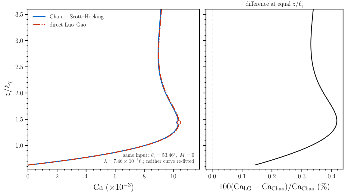
Figure 3: Full-formulation comparison at identical microscopic inputs: \theta_e = 53.46^\circ , \mu_r = 0 , and \lambda/\ell_\gamma = 7.46 \times 10^{-6} , with neither equation re-fitted. Left: the Chan equation with the Scott-Hocking closure and the direct Luo-Gao equation. Right: their relative capillary-number difference at equal meniscus rise. The direct Luo-Gao fold is 0.41690% above the Chan fold for this common input; the difference includes both the matching constants and the local viscous terms.
