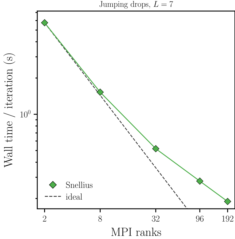
Figure 9: Strong scaling of the uniform-grid jumping-drop kernel on Snellius Genoa. Full octree at L = 7 . The serial STL reconstruction writes a dump that the MPI ranks restore before the timed window; the ten solver steps themselves write no output.
