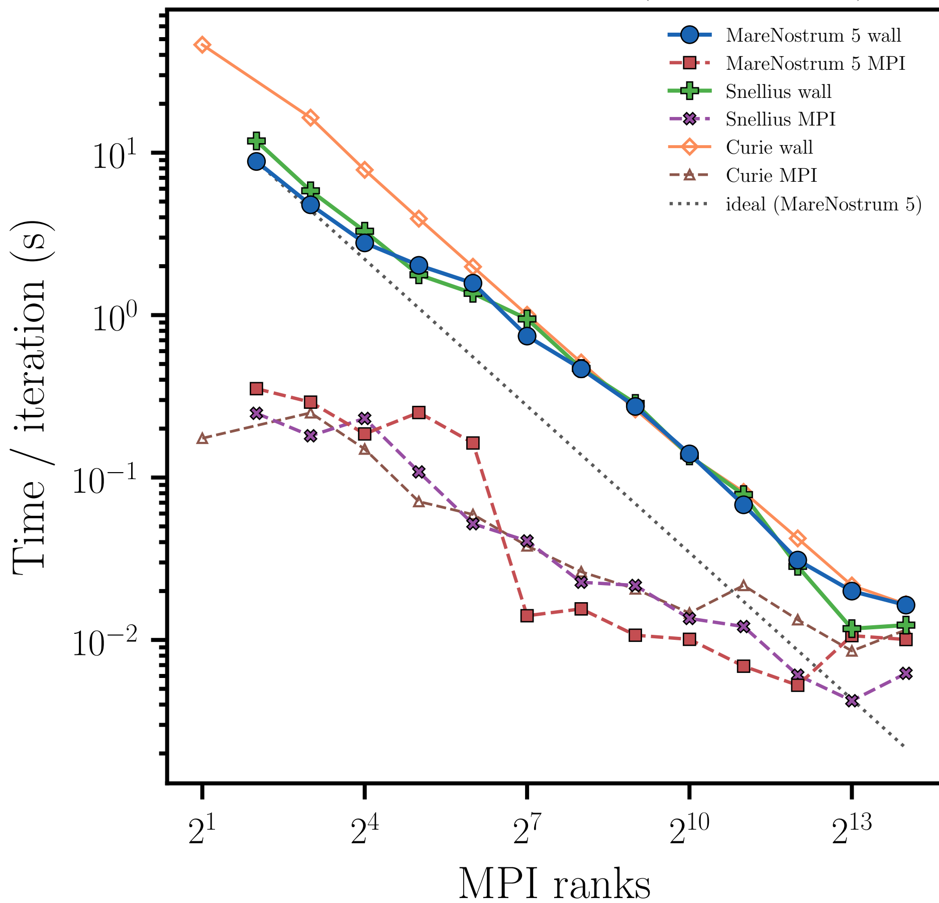
Poisson, 2D full quadtree L = 14 (Curie comparison)
