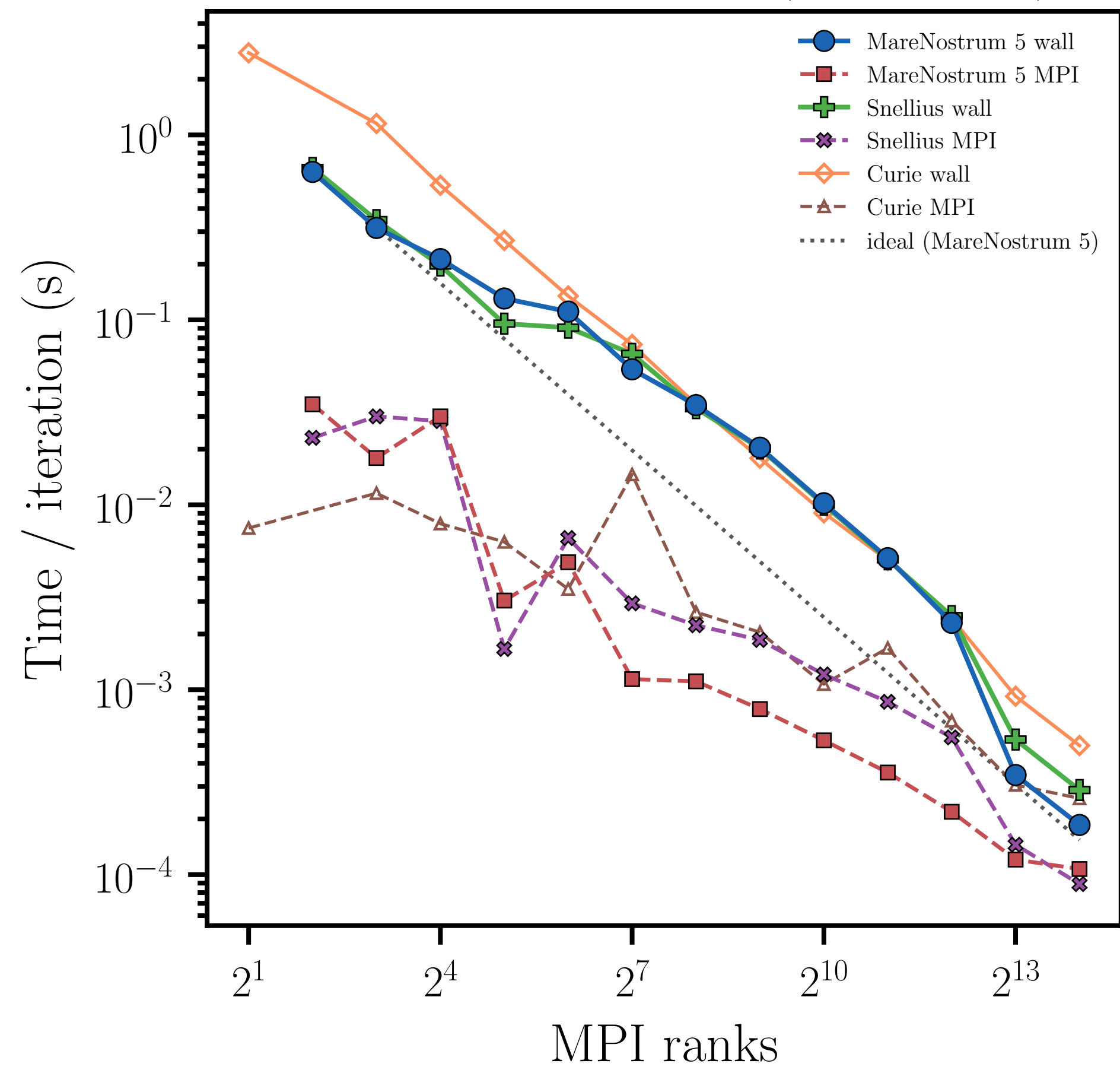
Laplacian, 2D full quadtree L = 14 (Curie comparison)
