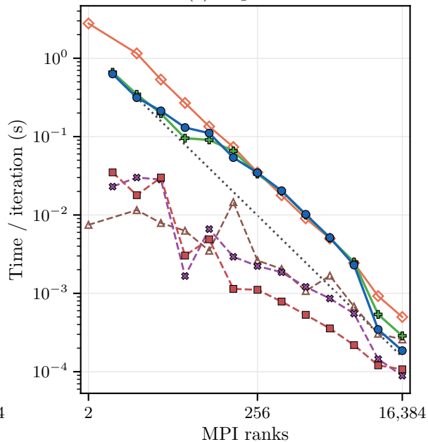
(b) Laplacian
