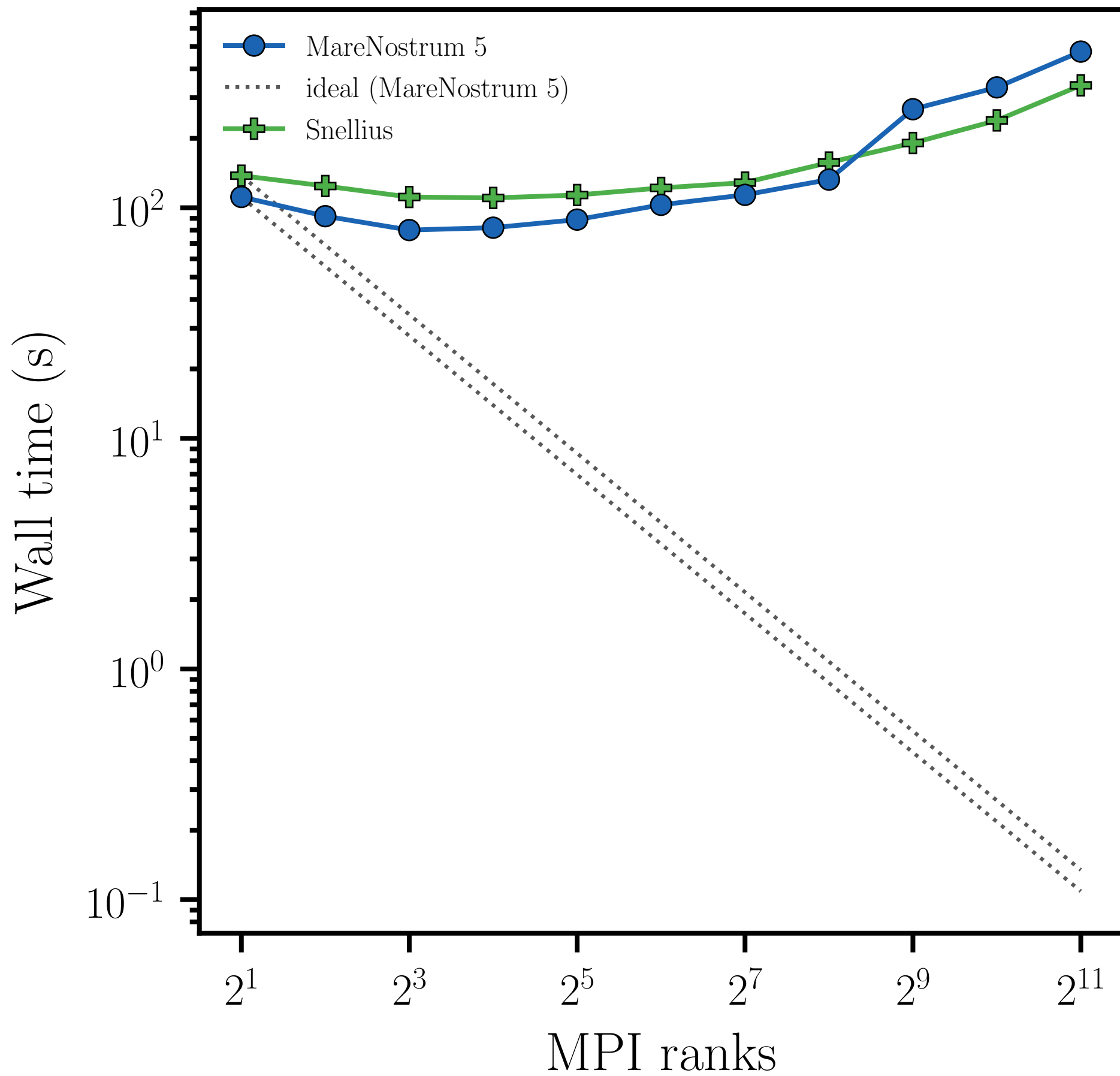
Marangoni migration, L = 10 (64 pts/ R )
