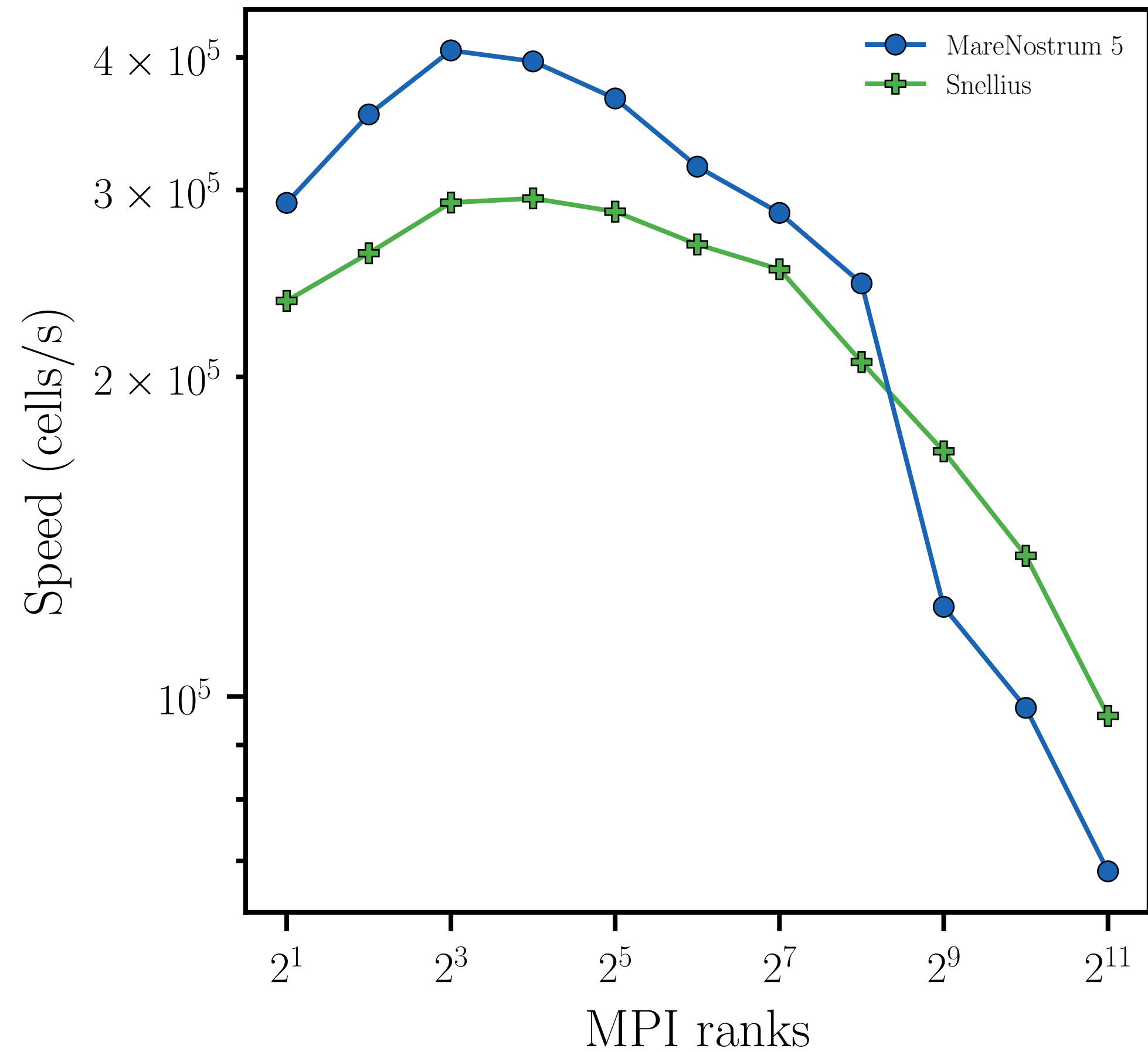
Marangoni migration, L = 10 (64 pts/ R )
