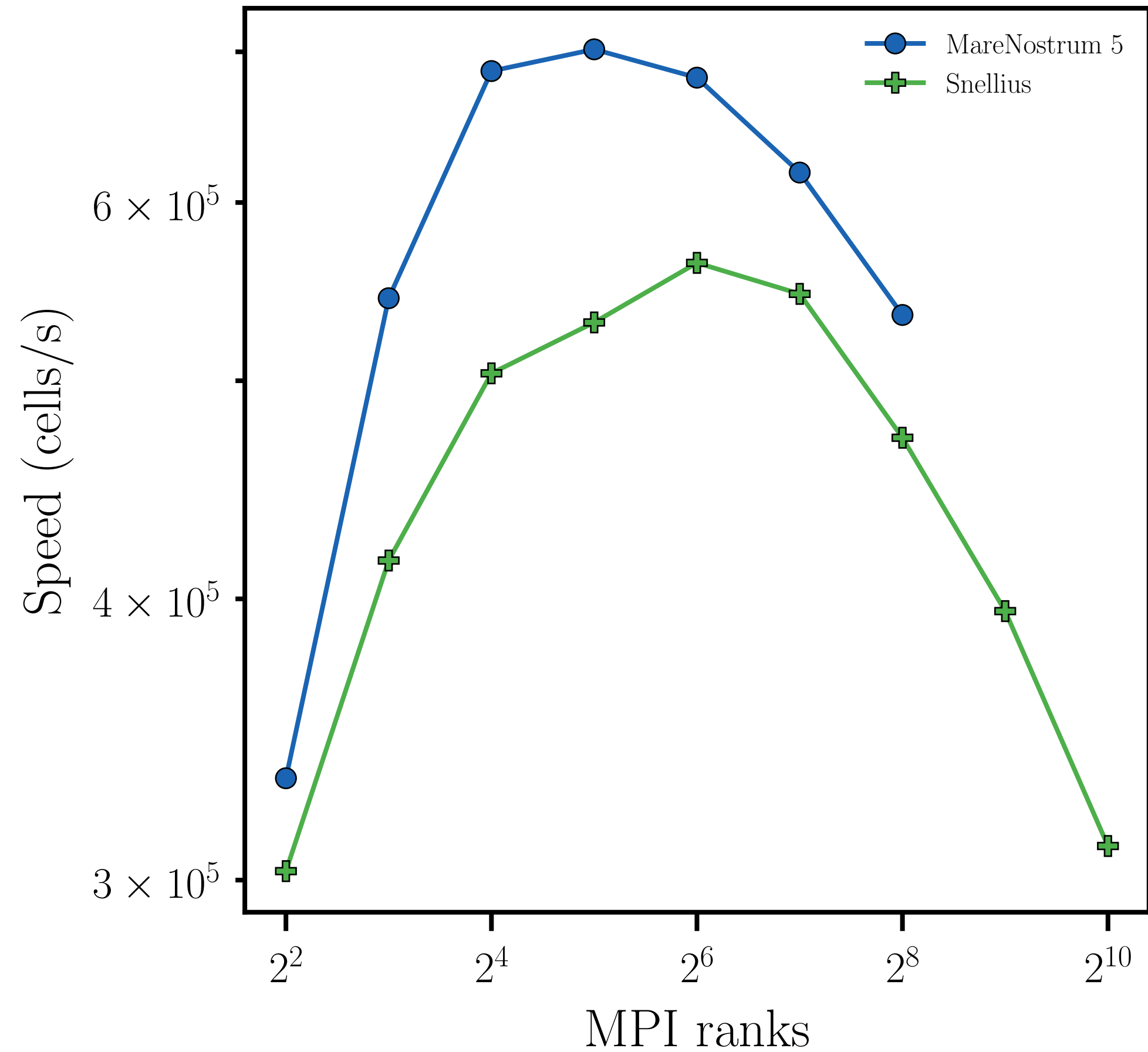
Marangoni migration, L = 12 (256 pts/ R )
