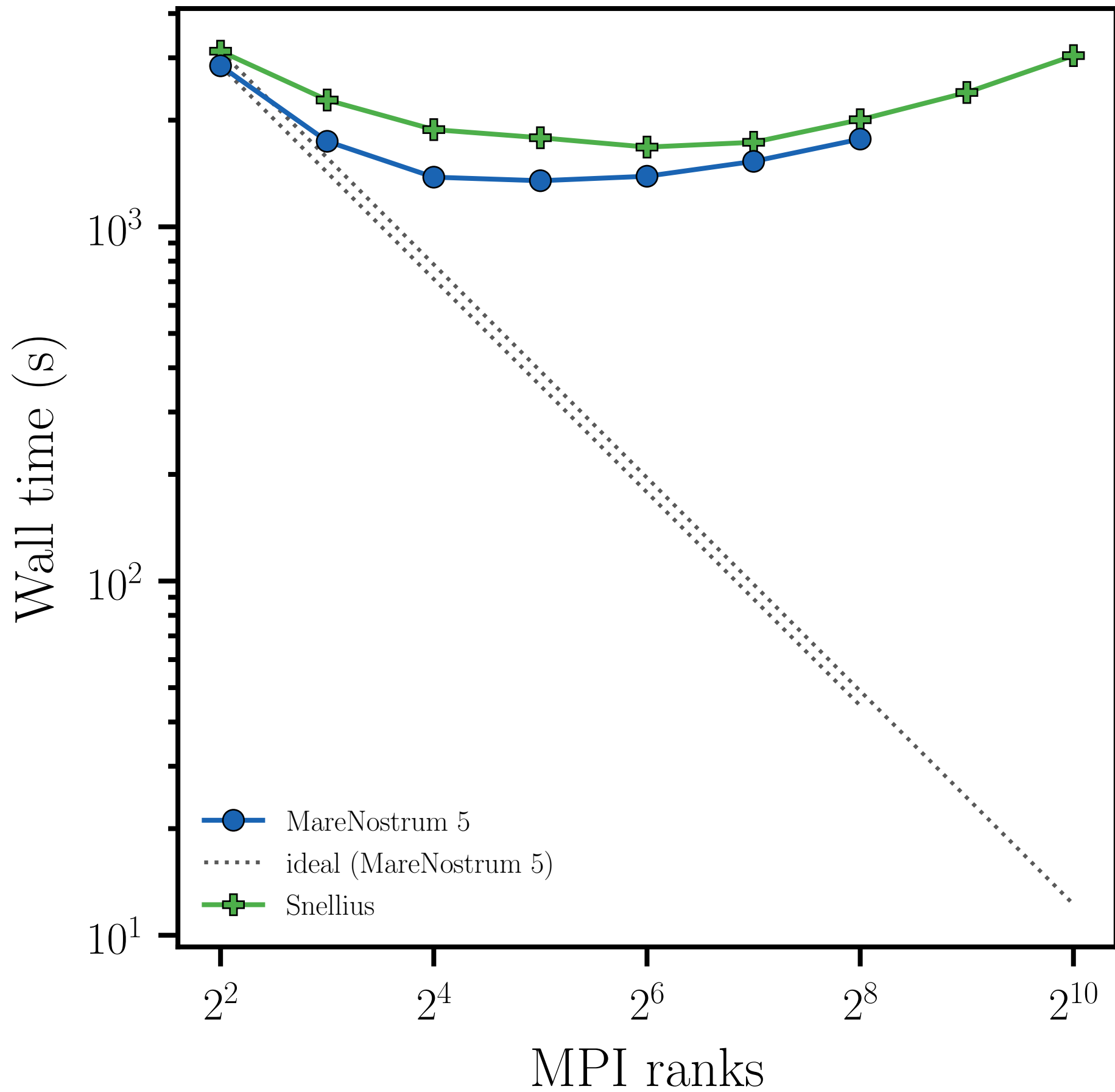
Marangoni migration, L = 12 (256 pts/ R )
