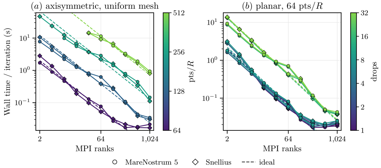
Figure 3: Active-drop scaling in the abundant-fuel limit on MareNostrum 5 GPP (circles) and Snellius Genoa (diamonds). (a) Axisymmetric uniform meshes at 64–512 points per radius. (b) Planar workloads with 1–32 drops at 64 points per radius. Dashed lines show ideal scaling.
