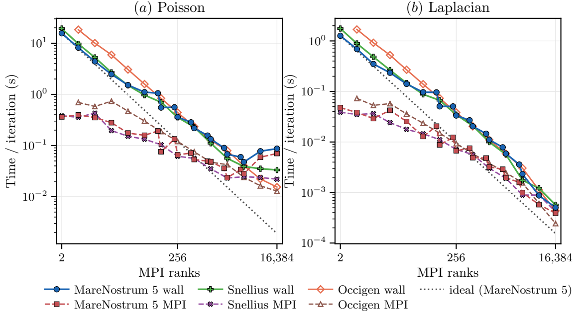
Figure 2: Strong scaling of the stock three-dimensional mpi-laplacian test on a full octree at L = 9 . (a) Poisson solve. (b) Laplacian operator. Solid and dashed curves show wall and MPI time per iteration, respectively. Occigen data provide the stock reference; the dotted line gives ideal scaling from the MareNostrum 5 baseline.
