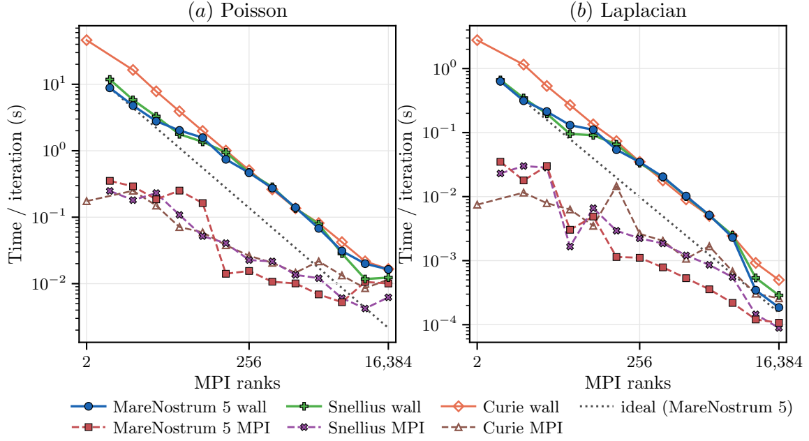
Figure 1: Strong scaling on a full two-dimensional quadtree at L = 14 . (a) Poisson solve. (b) Laplacian operator. Solid curves show wall time per iteration; dashed curves show the measured MPI contribution. The grey dotted line follows ideal scaling from the MareNostrum 5 baseline. Curie data are distributed with the stock Basilisk test.
