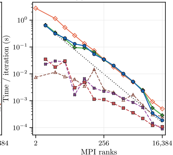
(b) Laplacian
