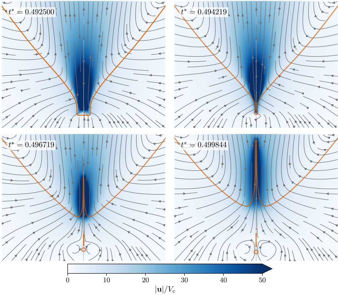
Figure 4: Bursting bubble. (a) Snellius Genoa strong scaling of the axisymmetric uniform-grid kernel; colour gives N_x = 2^L and dashed corner guides show ideal scaling. (b) Jet inception at Oh = 0.03 , Bo = 0 . Blue gives |\mathbf{u}|/V_c , where V_c = \sqrt{\sigma/(\rho_l R)} and t^* = tV_c/R ; grey curves are instantaneous streamlines and orange marks the interface. The sequence shows the narrowing cavity, emerging jet and entrapped bubble. Colours saturate above 50V_c .
