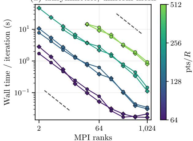
(a) axisymmetric, uniform mesh
