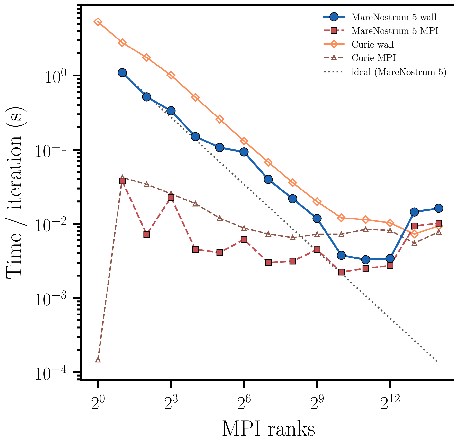
Poisson, 2D full quadtree L = 12 (Curie comparison)
