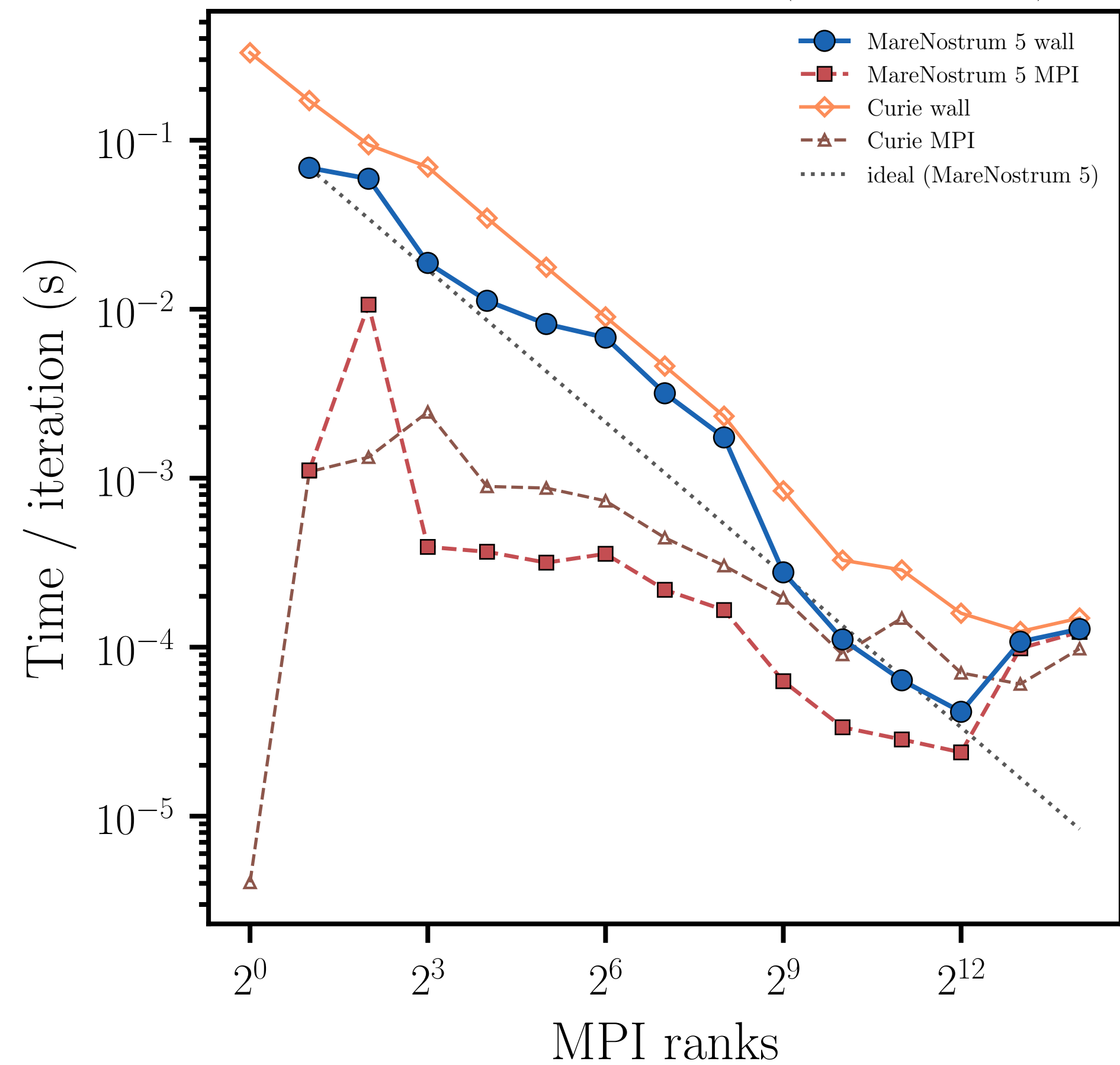
Laplacian, 2D full quadtree L = 12 (Curie comparison)
