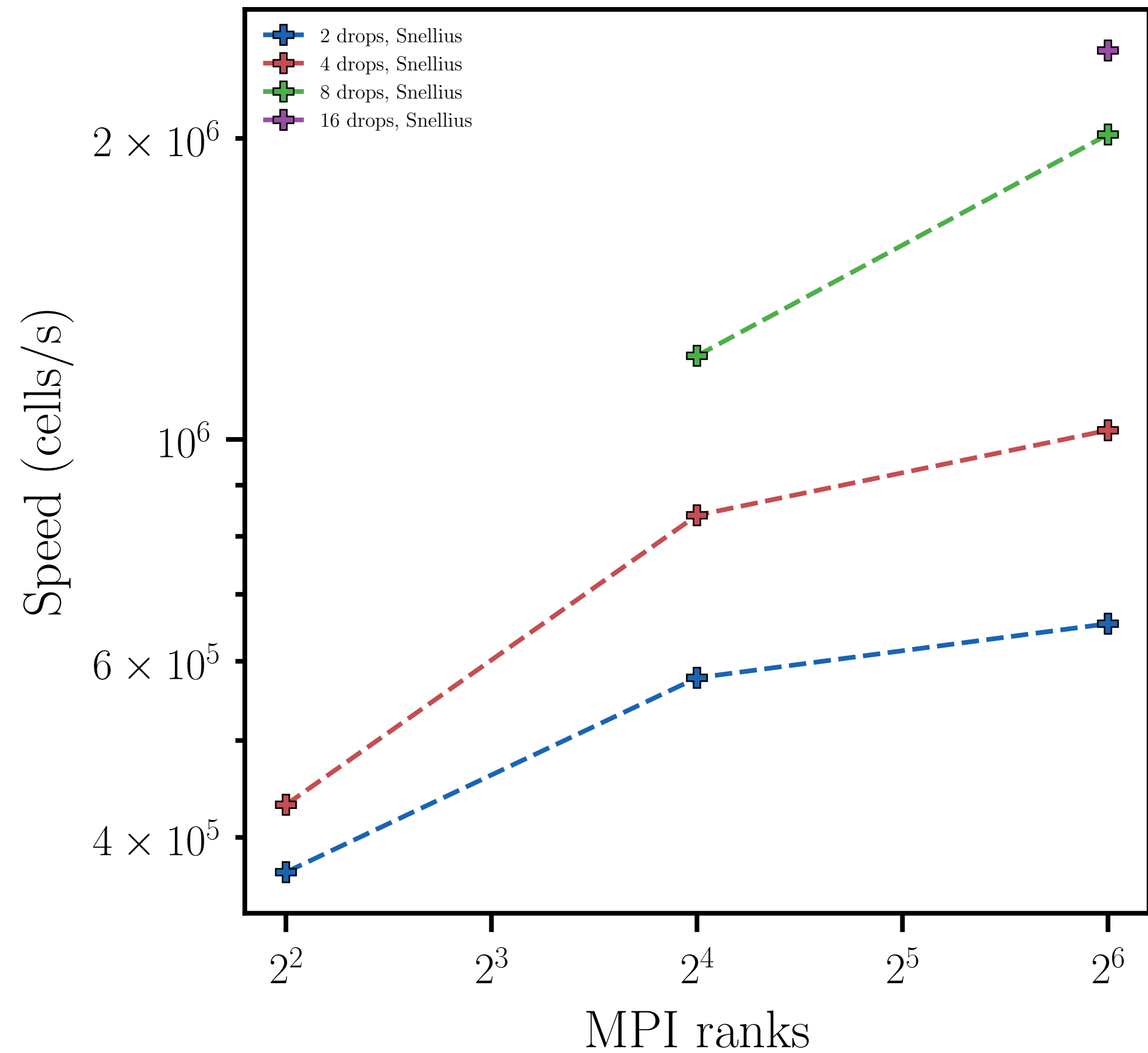
Planar multi-drop Marangoni, 64 pts/ R
