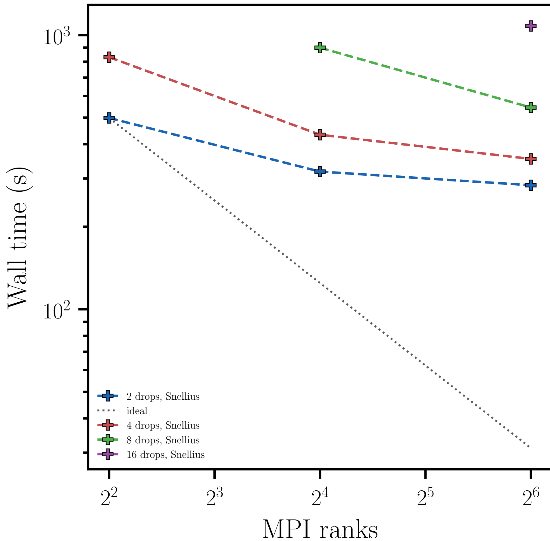
Planar multi-drop Marangoni, 64 pts/ R
