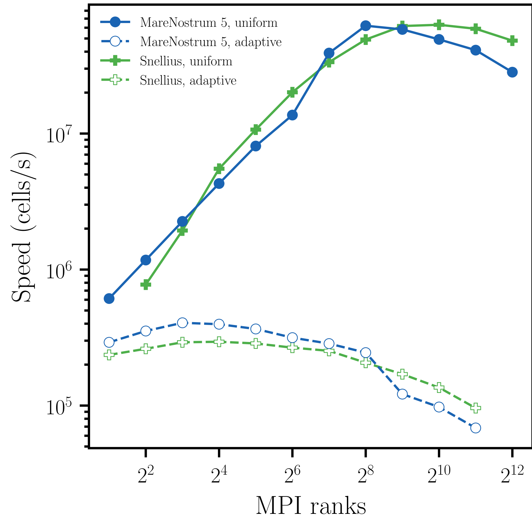
Marangoni migration, adaptive vs uniform, L = 10 (64 pts/ R )
