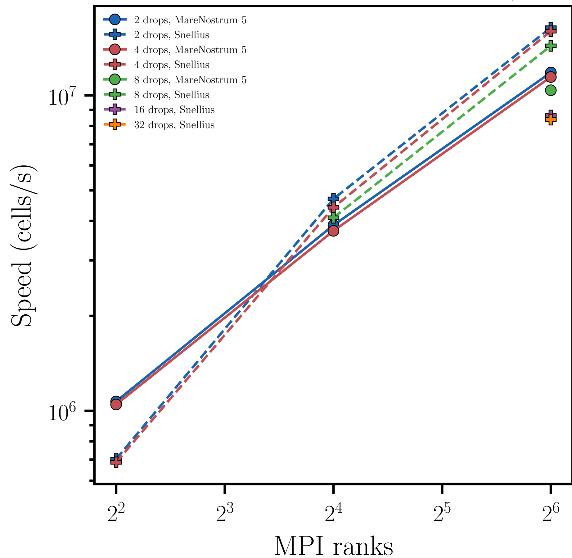
Planar multi-drop Marangoni, uniform mesh, 64 pts/ R
