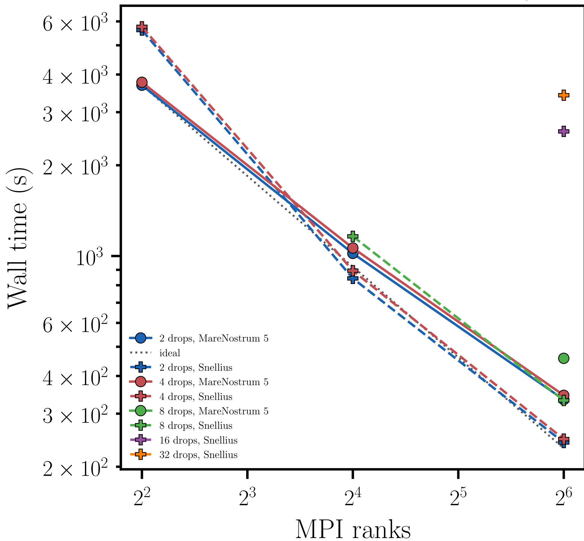
Planar multi-drop Marangoni, uniform mesh, 64 pts/ R
