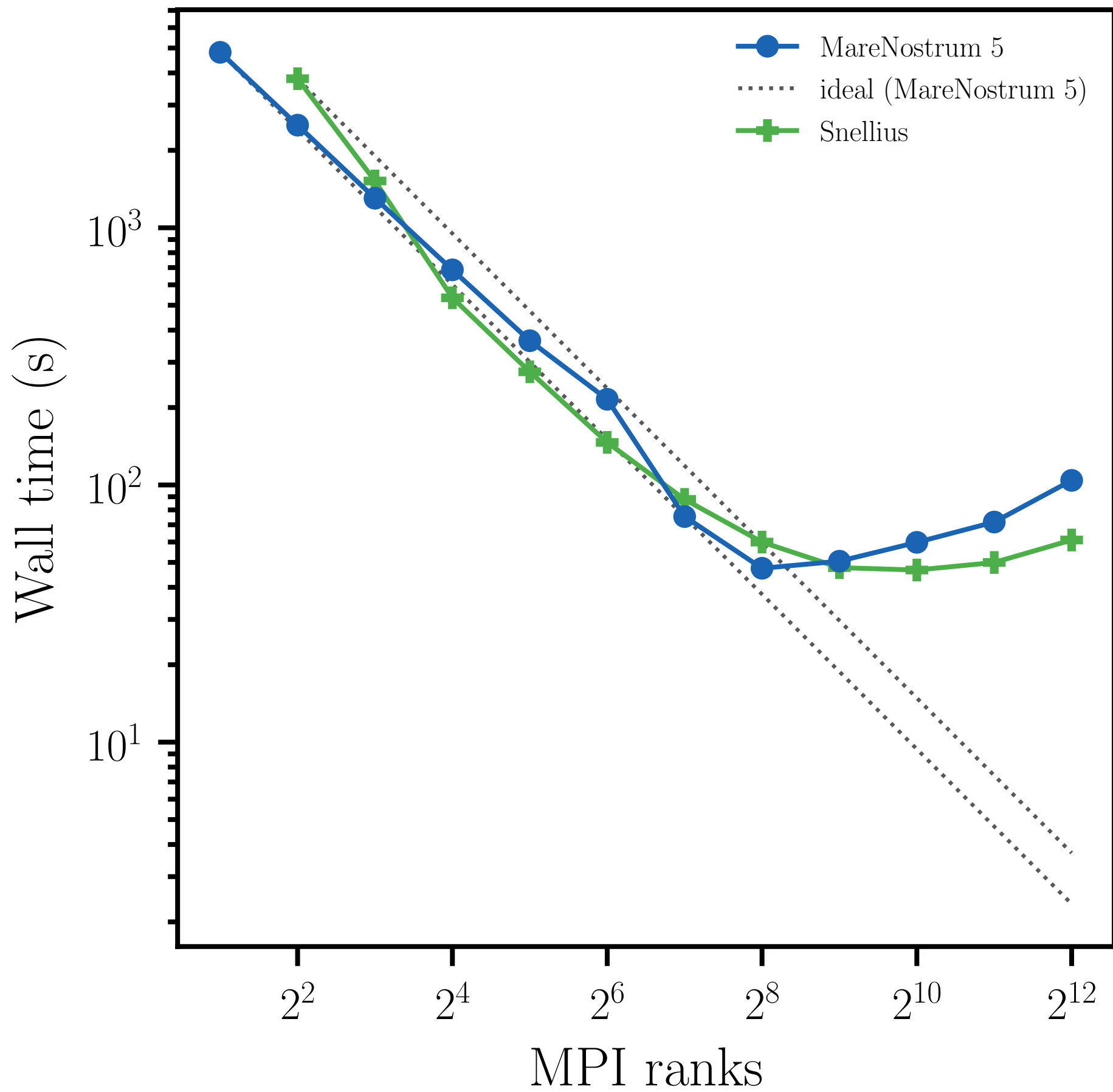
Marangoni migration, uniform mesh, L = 10 (64 pts/ R )
