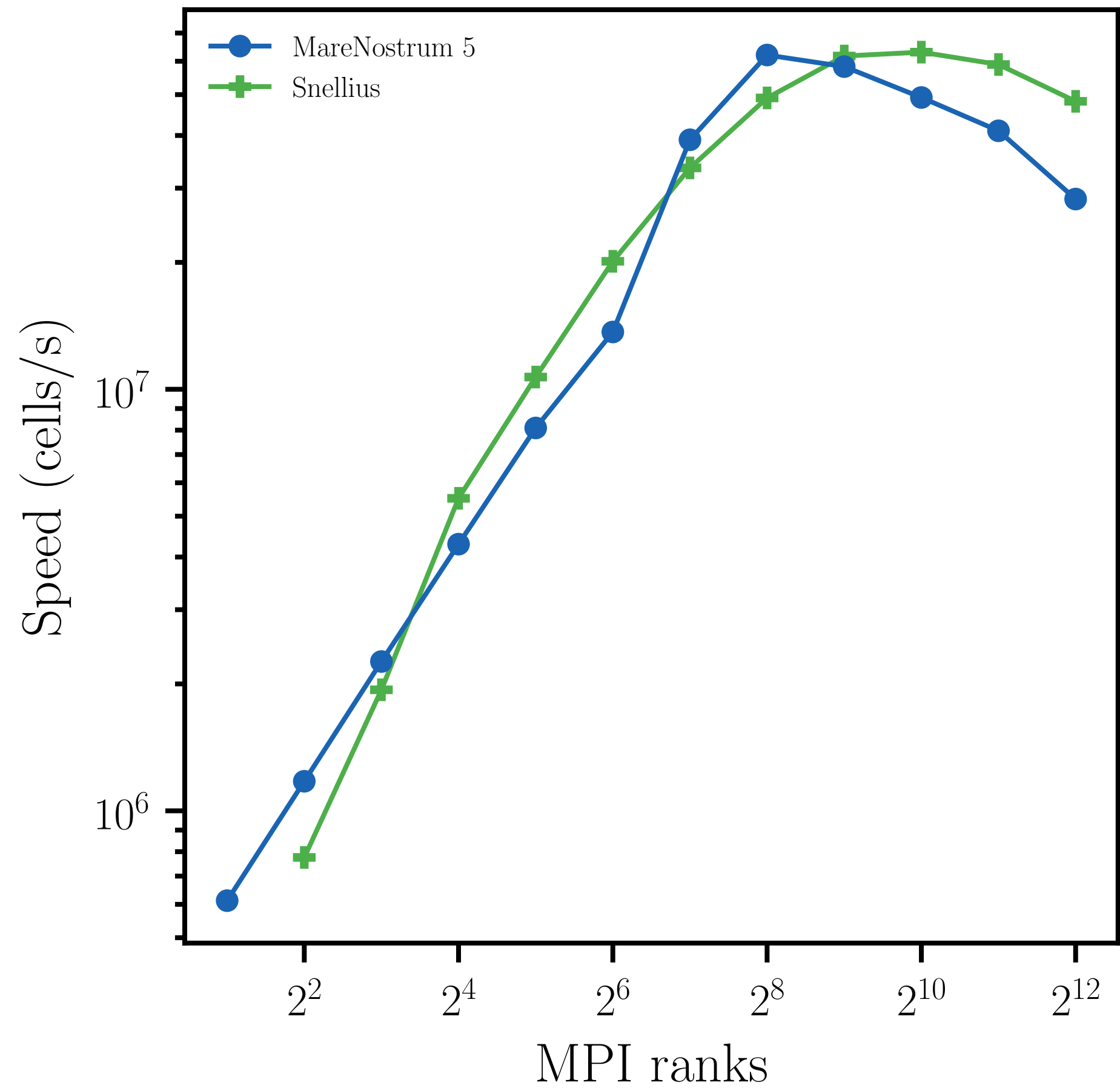
Marangoni migration, uniform mesh, L = 10 (64 pts/ R )
