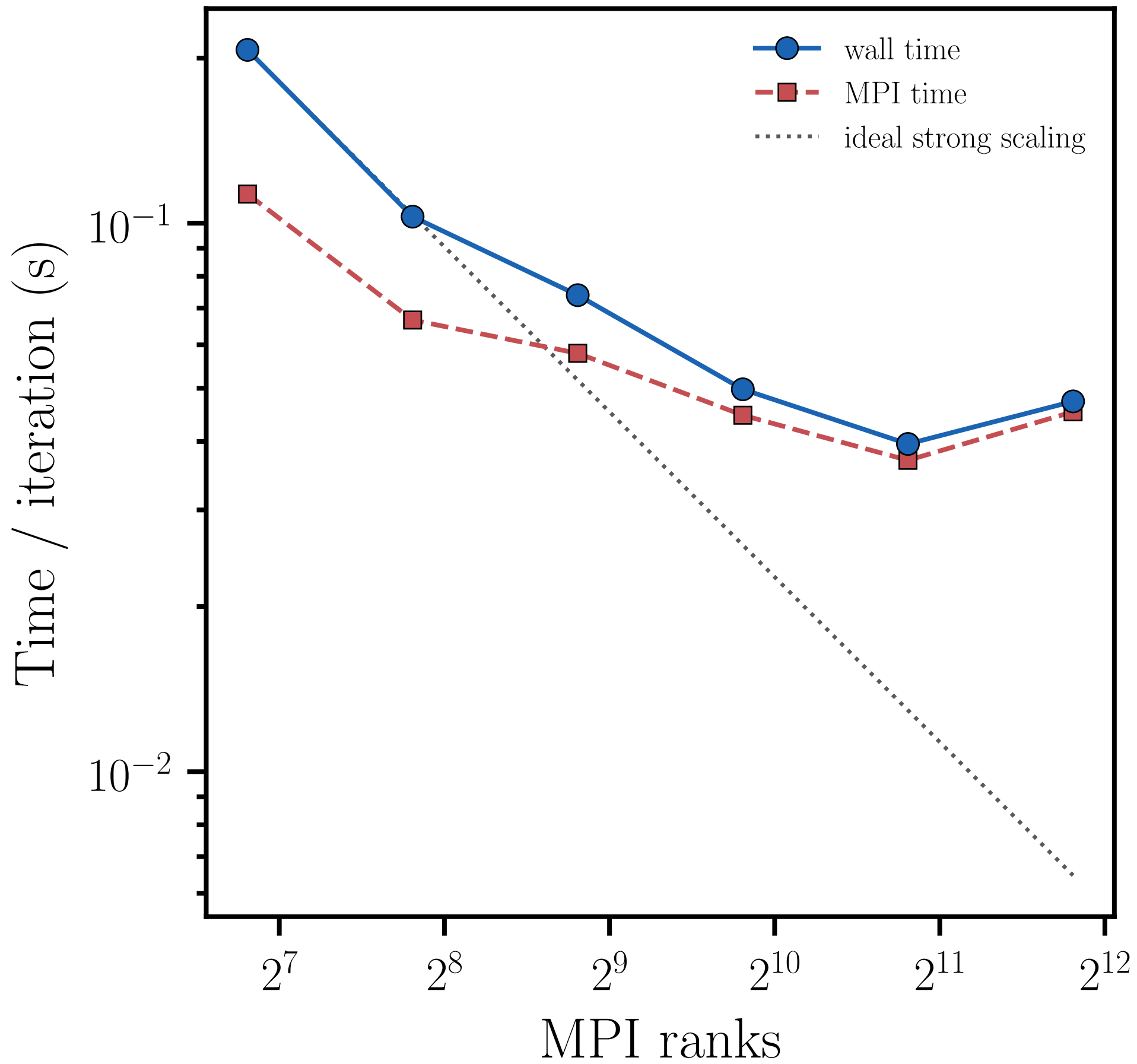
Poisson, stock mpi-circle, adaptive L = 14
