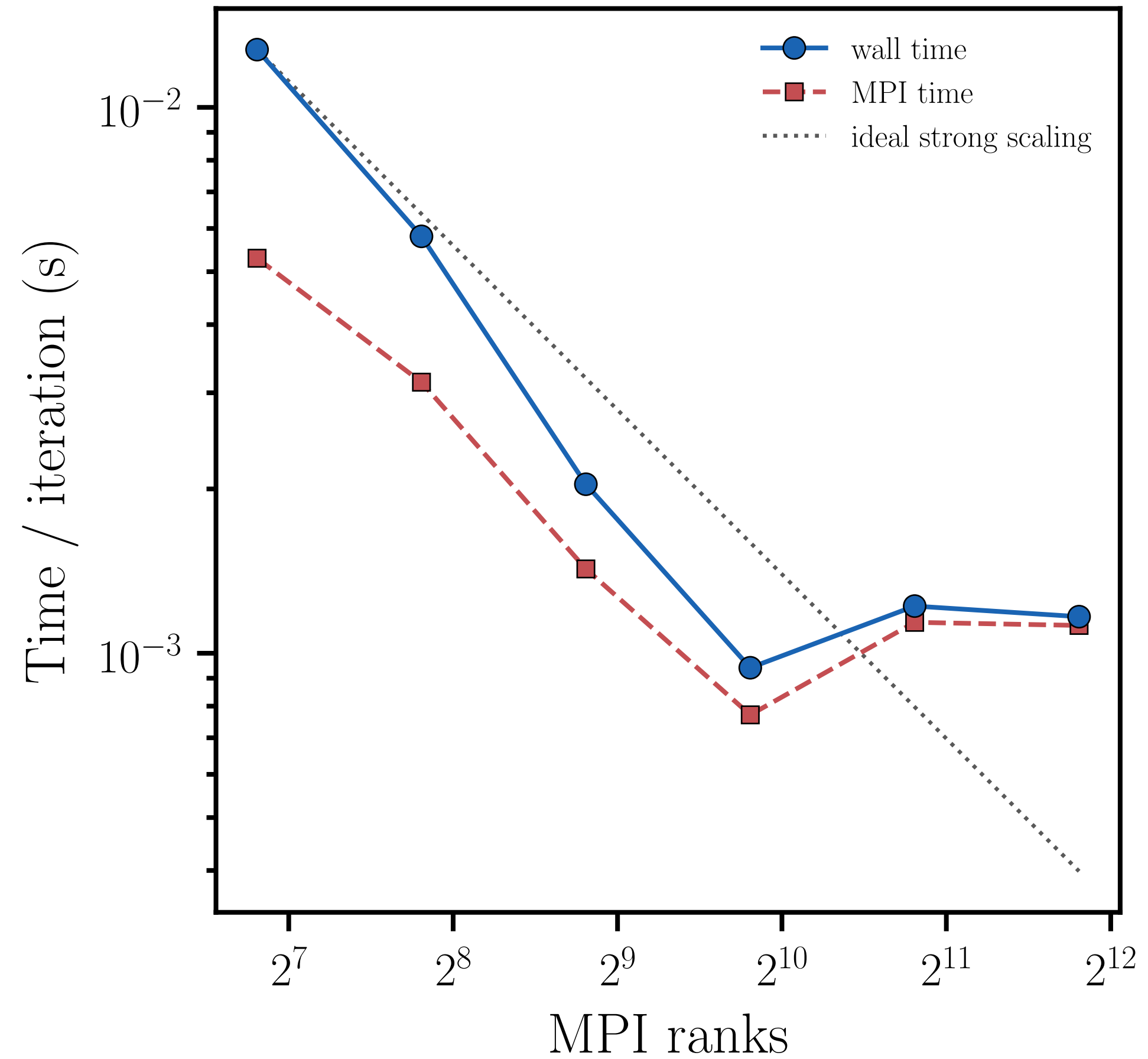
Laplacian, stock mpi-circle, adaptive L = 14
