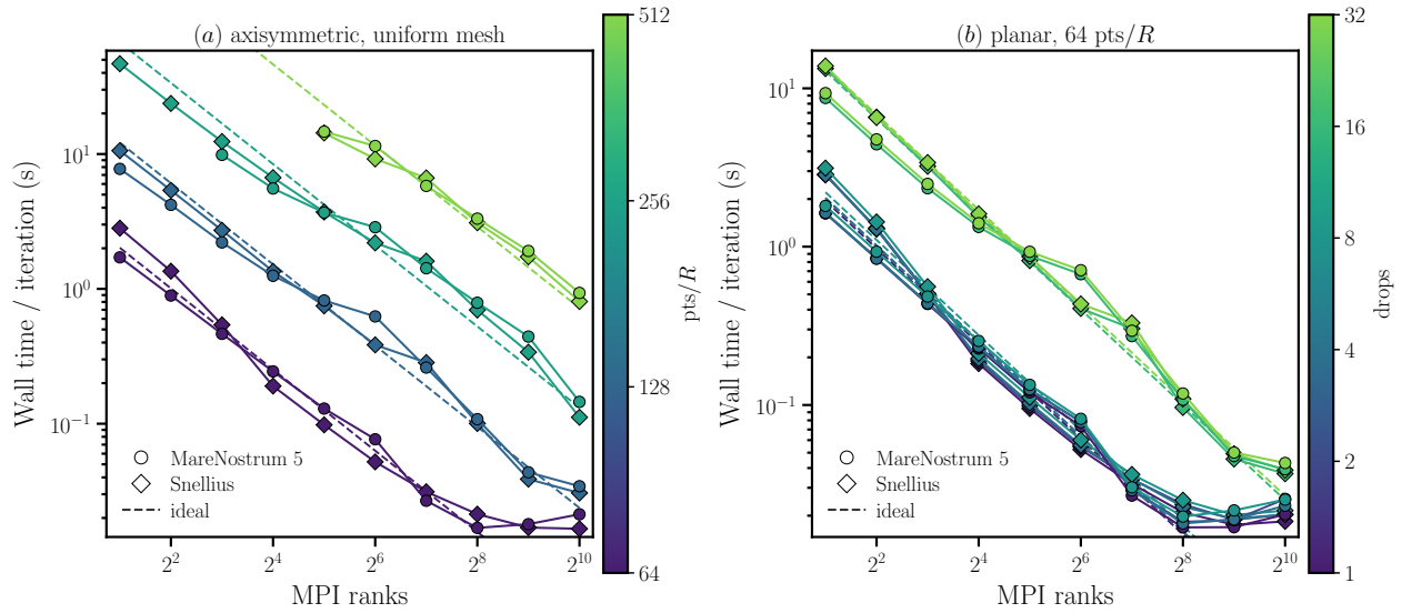
Figure 1: Abundant-fuel active-drop scaling on MareNostrum 5 GPP (circles) and Snellius Genoa (diamonds). (a) Uniform meshes at 64–512 points per radius. (b) Planar 1–32-drop workloads at 64 points per radius. Dashed lines show ideal scaling. Each point is one recorded run; the current tables do not measure run-to-run variability.
