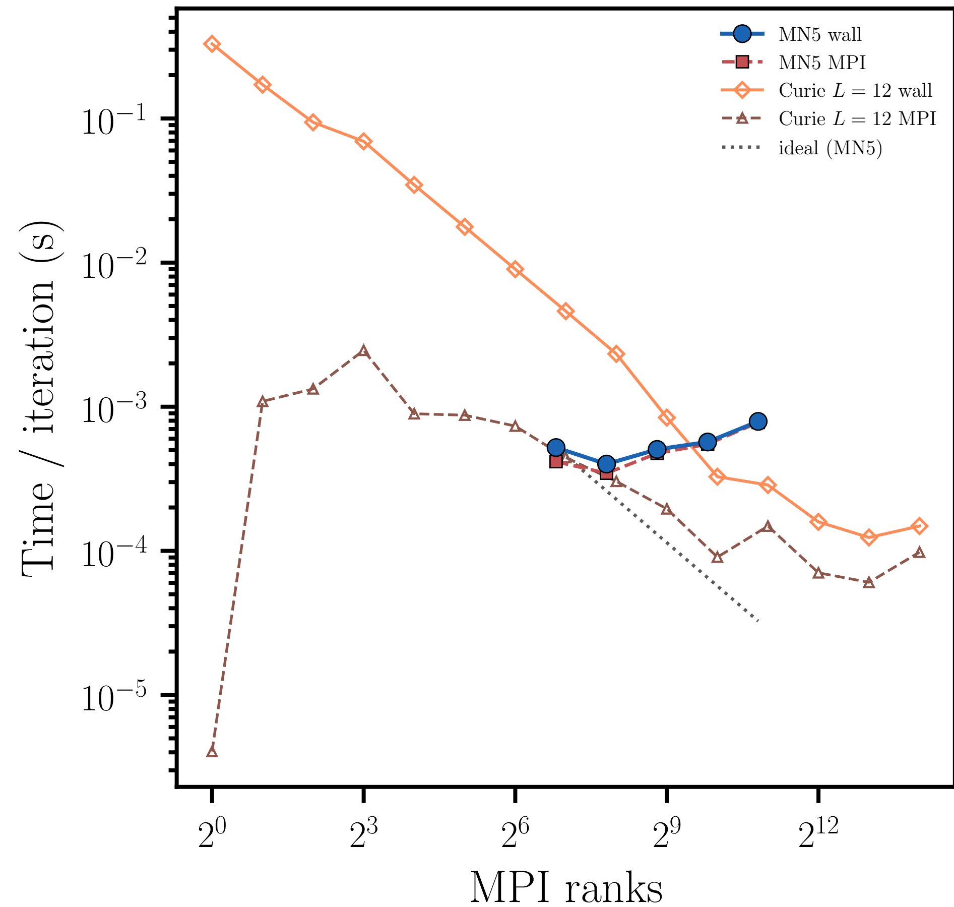
Laplacian, stock mpi-circle, adaptive L = 12
