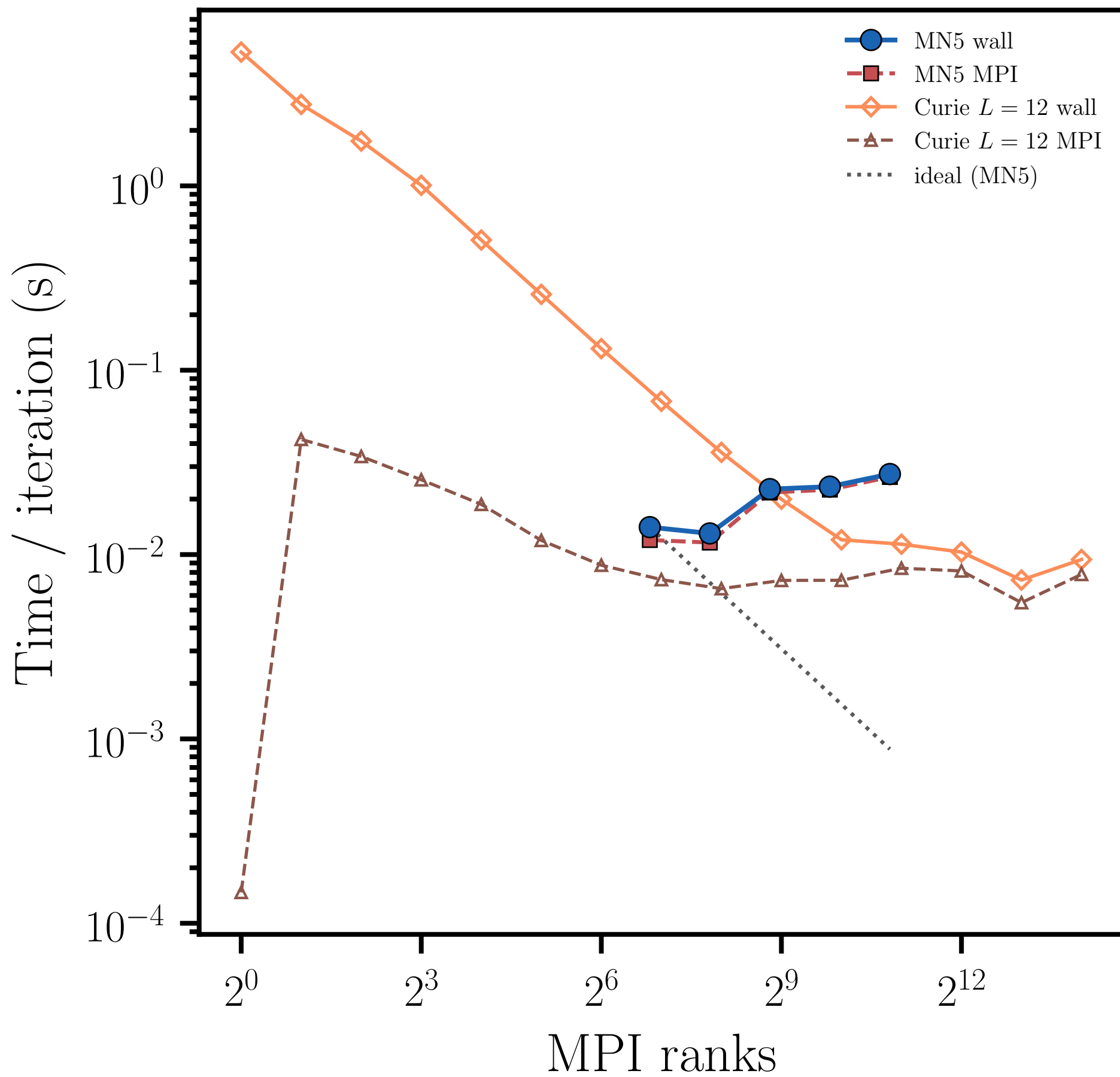
Poisson, stock mpi-circle, adaptive L = 12
