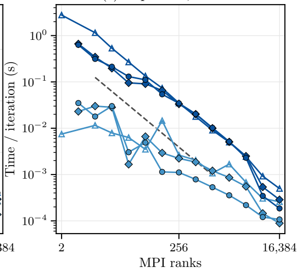
(b) Laplacian, L = 14
