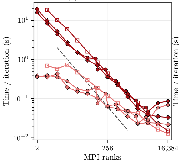
(c) Poisson, L = 9
