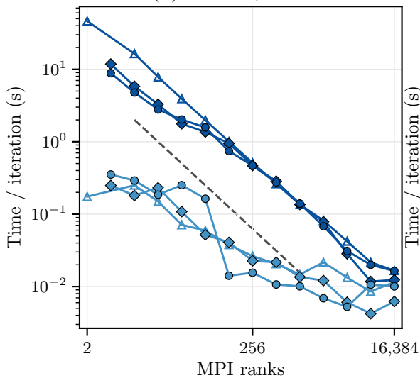
(a) Poisson, L = 14
