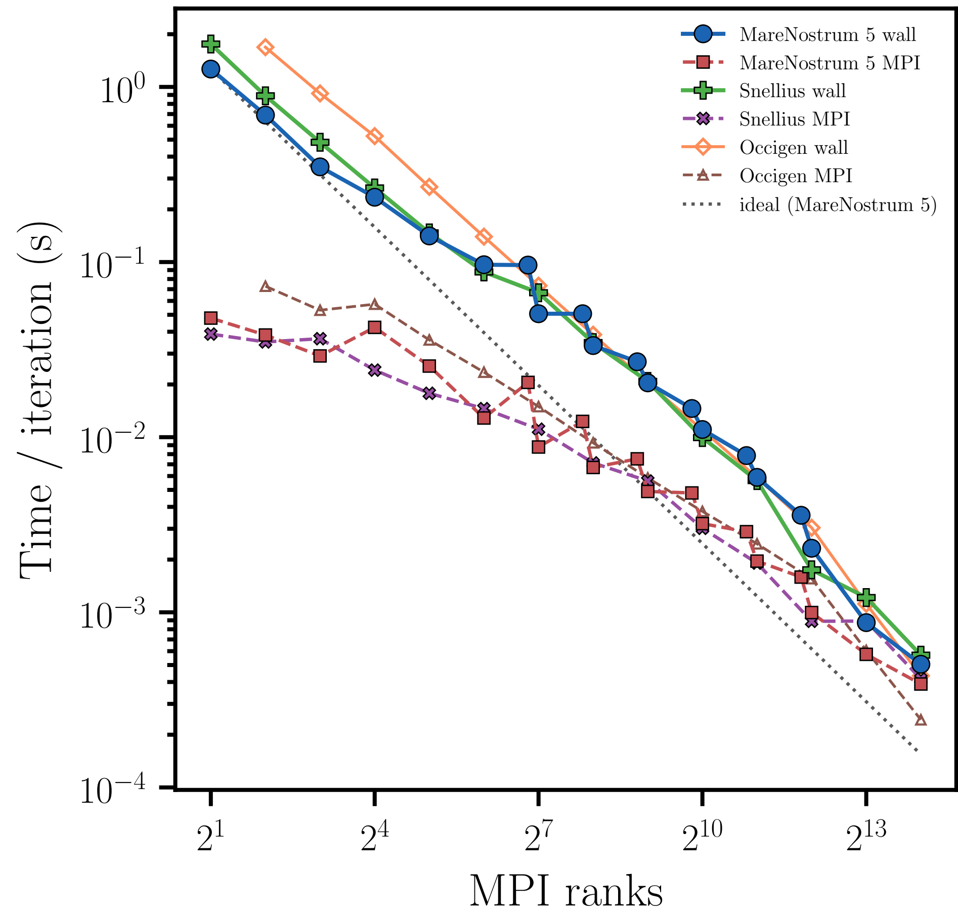
Laplacian, stock mpi-laplacian, octree L = 9
