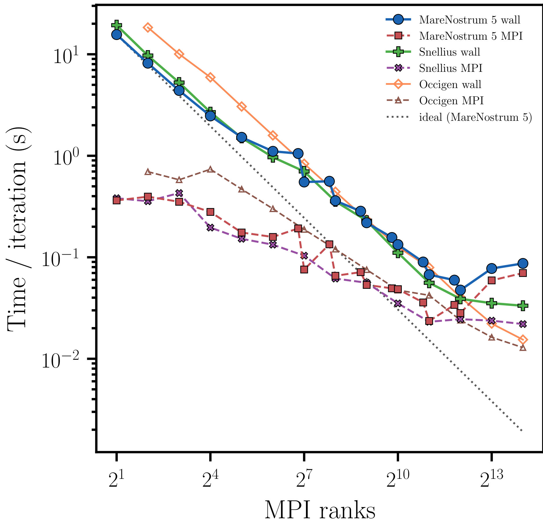
Poisson, stock mpi-laplacian, octree L = 9
