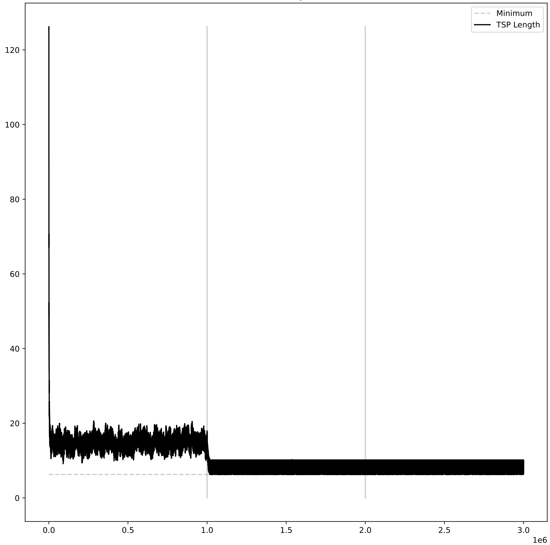
TSP convergence
