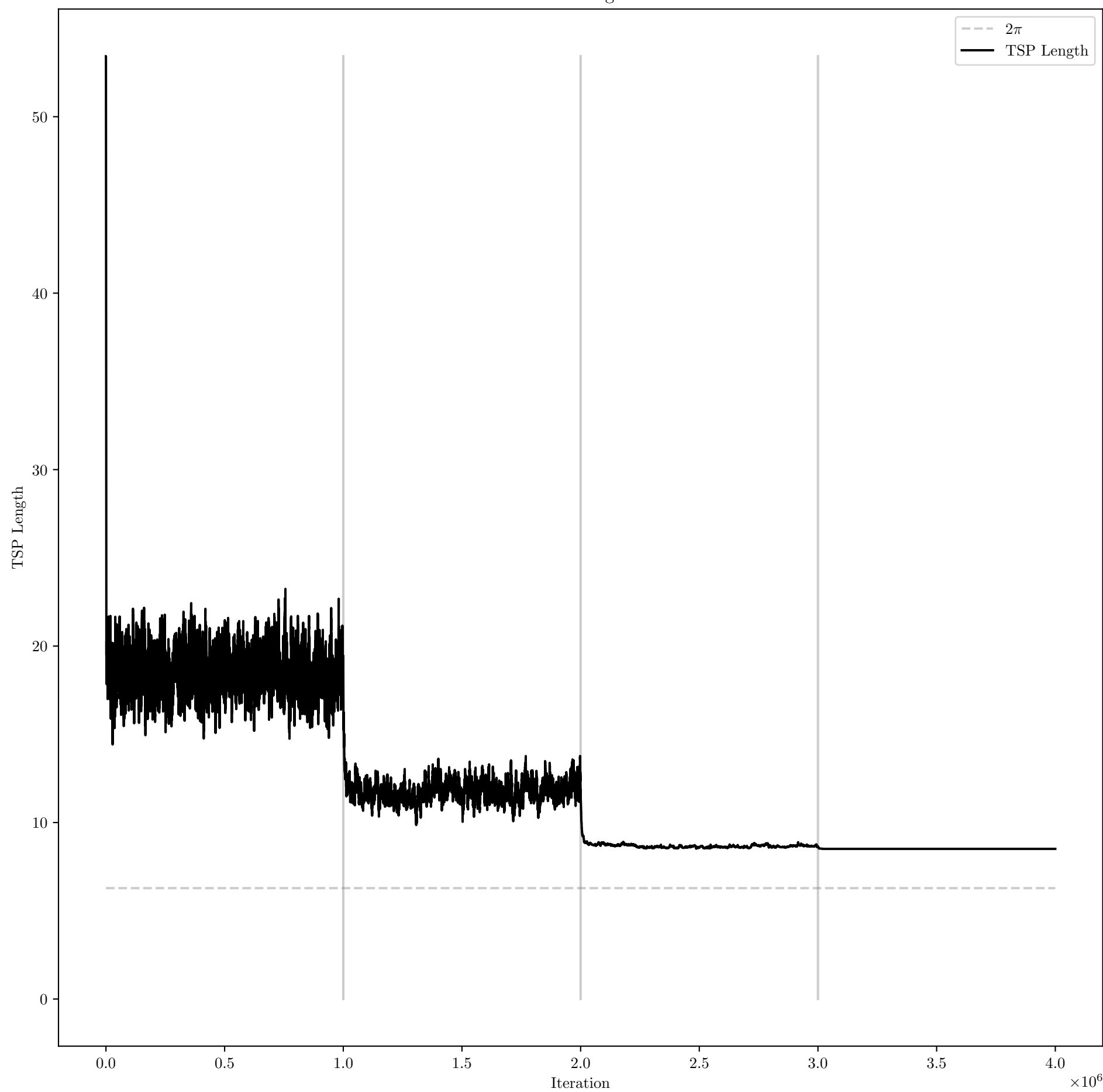
TSP convergence
