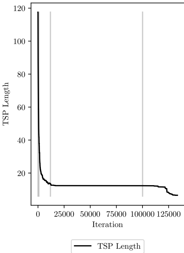
TSP cost evolution, final cost: 6.53
