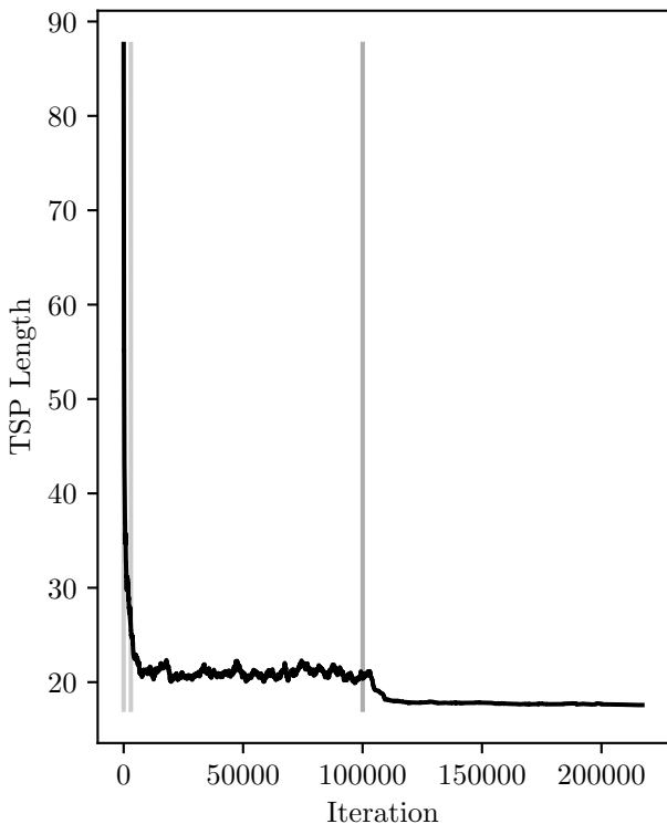
TSP cost evolution, final cost: 17.58
