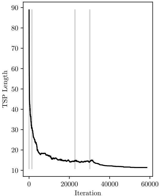
TSP cost evolution, final cost: 11.38
