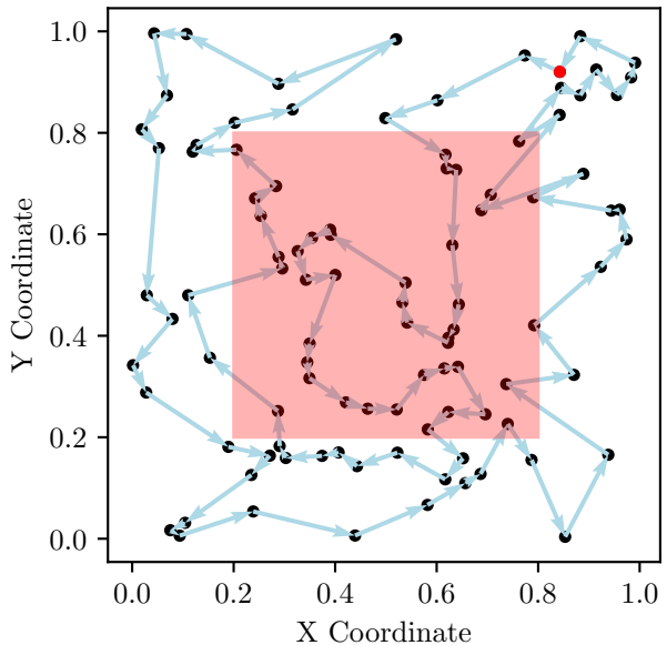
TSP Route, Cost: 9.76
