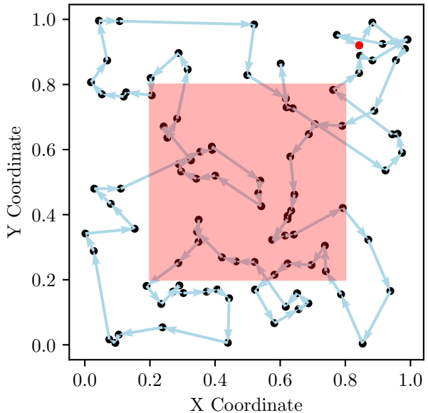
TSP Route, Cost: 9.33
