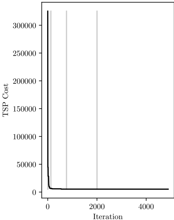
TSP cost evolution, final cost: 5215.56
