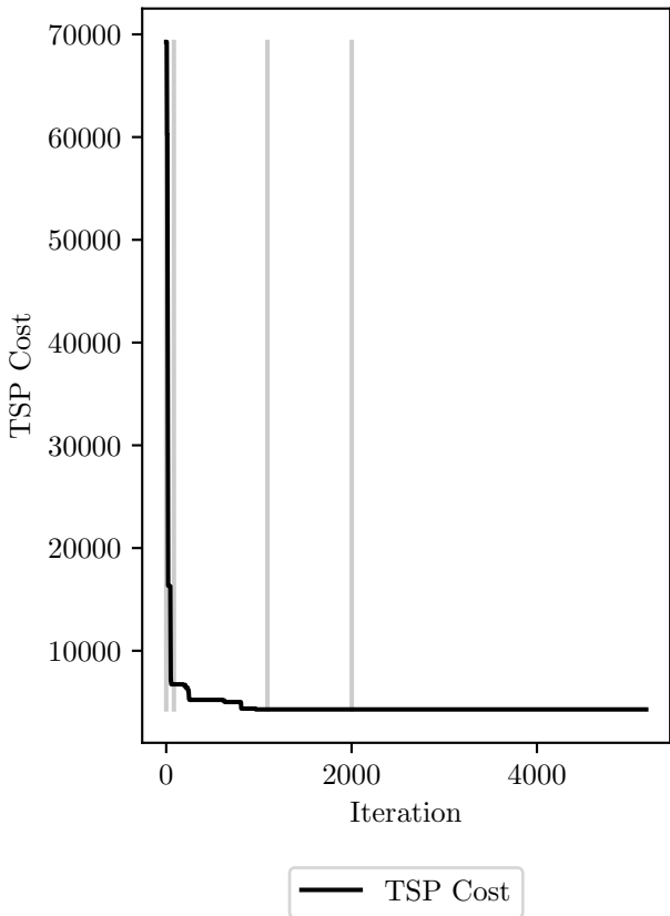
TSP cost evolution, final cost: 4290.88
