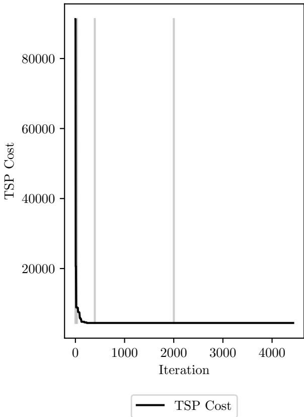
TSP cost evolution, final cost: 4452.81
