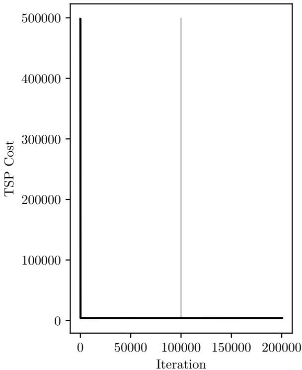
TSP cost evolution, final cost: 3873.14
