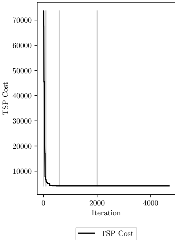
TSP cost evolution, final cost: 4159.23
