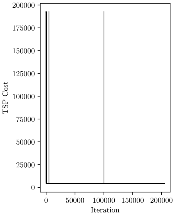
TSP cost evolution, final cost: 4229.32
