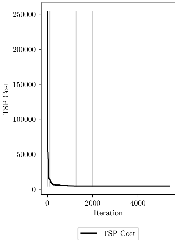
TSP cost evolution, final cost: 4434.09
