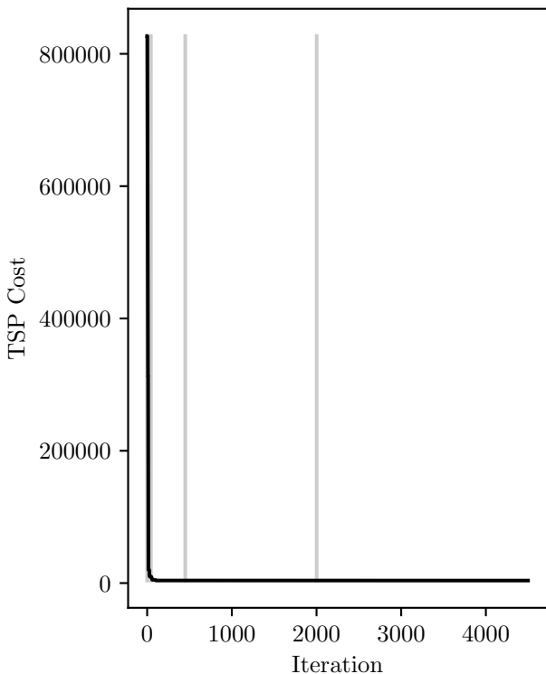
TSP cost evolution, final cost: 3804.94
