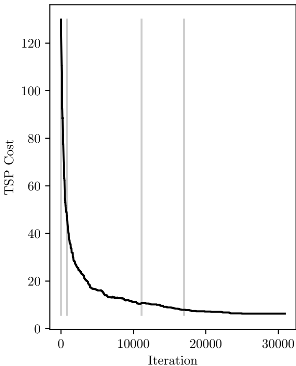
TSP cost evolution, final cost: 6.28
