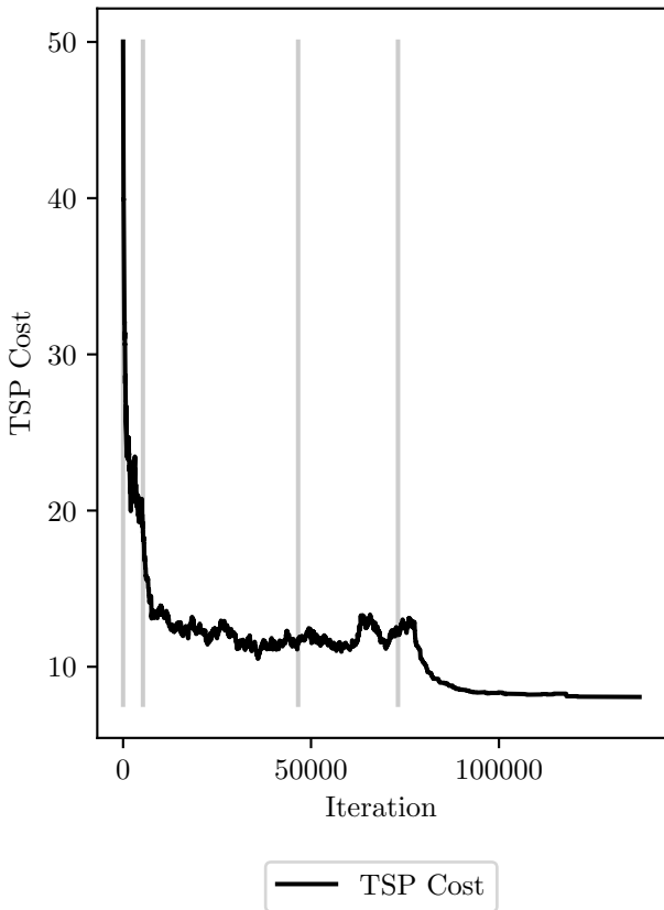
TSP cost evolution, final cost: 8.07
