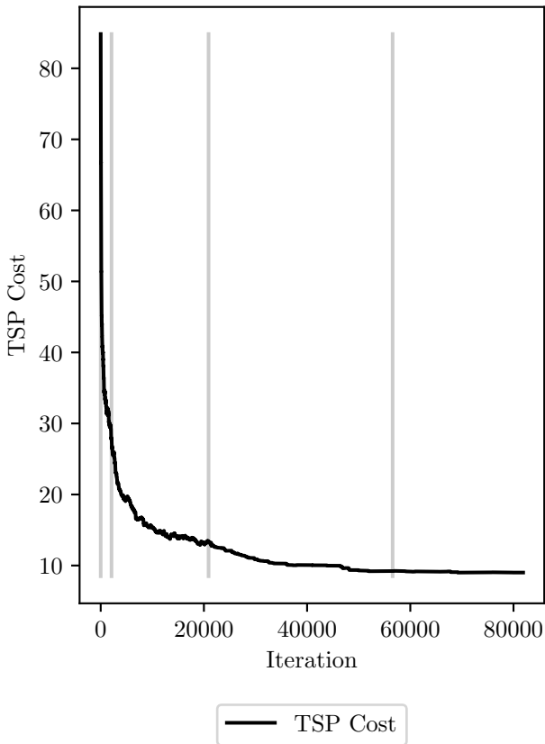
TSP cost evolution, final cost: 9.01
