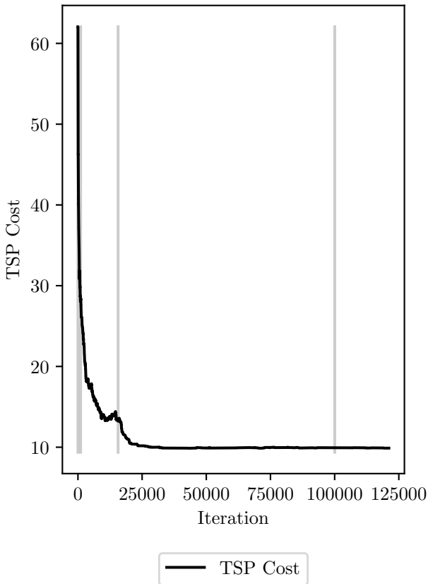
TSP cost evolution, final cost: 9.89
