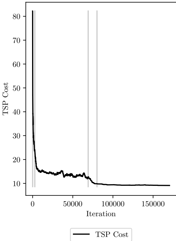
TSP cost evolution, final cost: 9.13
