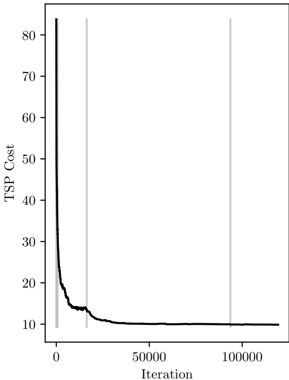
TSP cost evolution, final cost: 9.88
