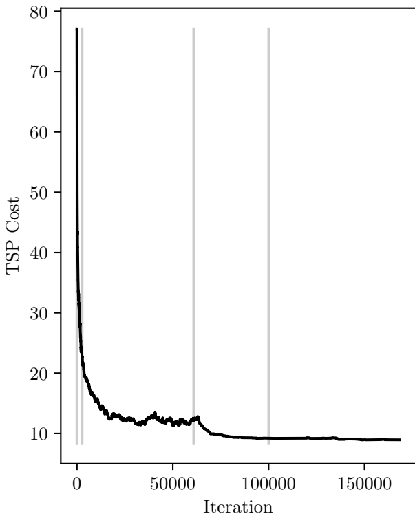
TSP cost evolution, final cost: 8.94
