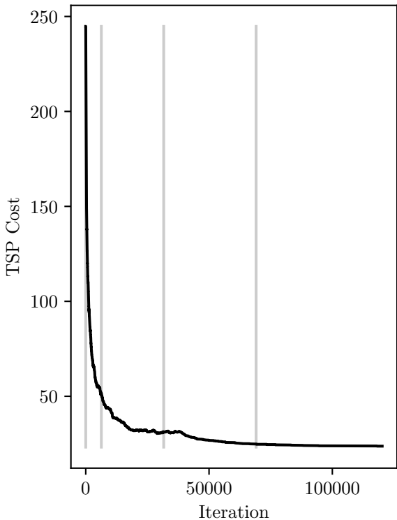
TSP cost evolution, final cost: 23.74
