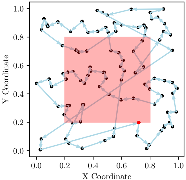
TSP Route, Cost: 16.33
