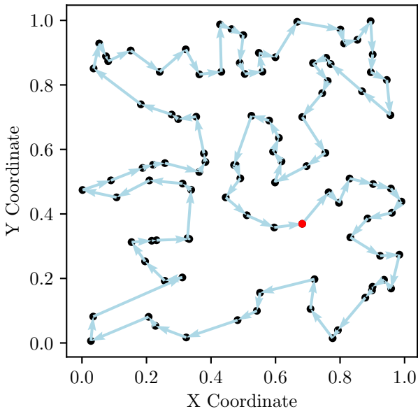
TSP Route, Cost: 7.93
