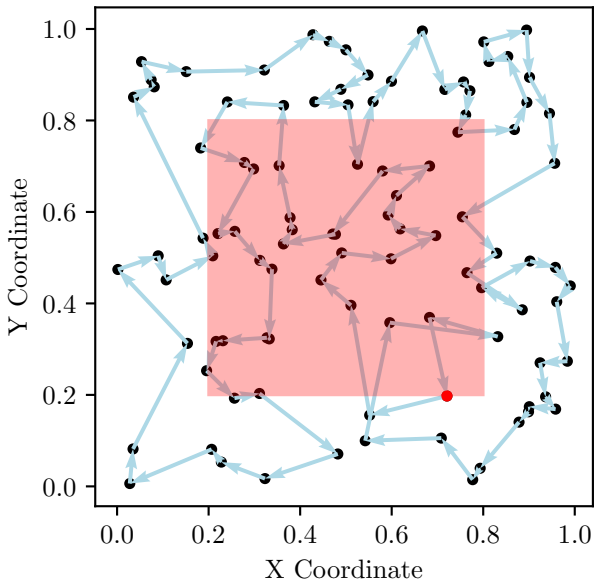
TSP Route, Cost: 9.89
