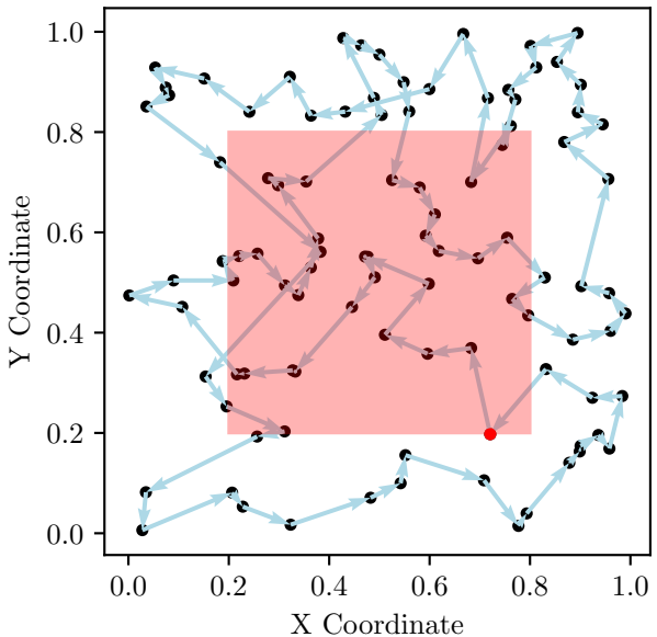
TSP Route, Cost: 9.13
