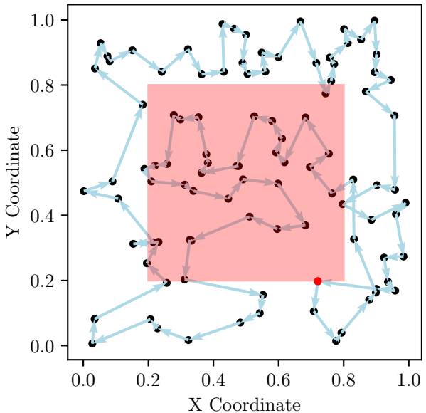
TSP Route, Cost: 9.17
